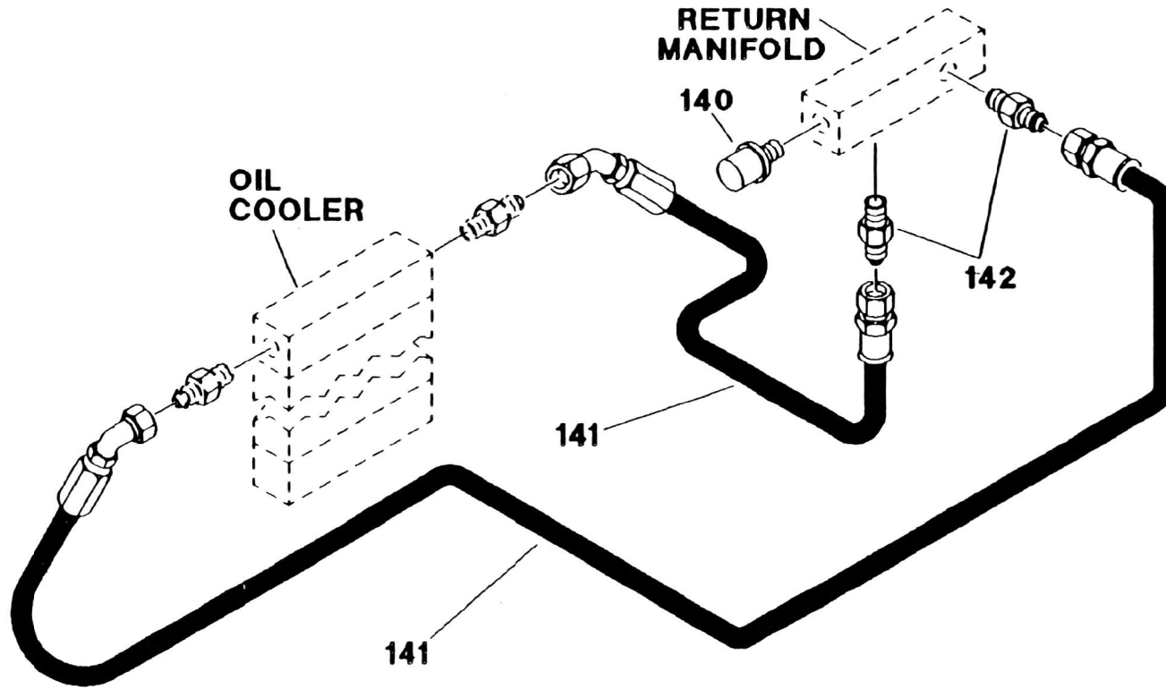
2140600090 HYD SCHEM - OIL COOLER J HOLLAR DEPT 530
